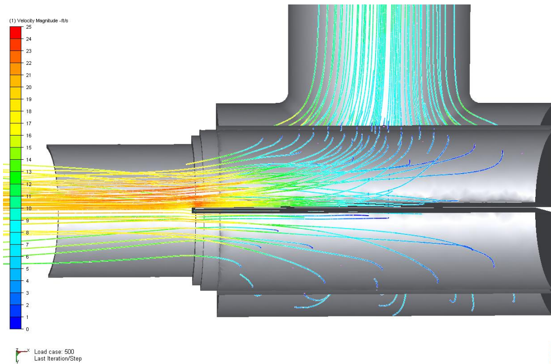
Figure 16. Fluid particle traces. (Cylindrical diffuser)
