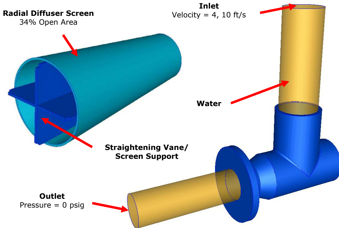
Figure 1. CFdesign analysis setup conditions.
