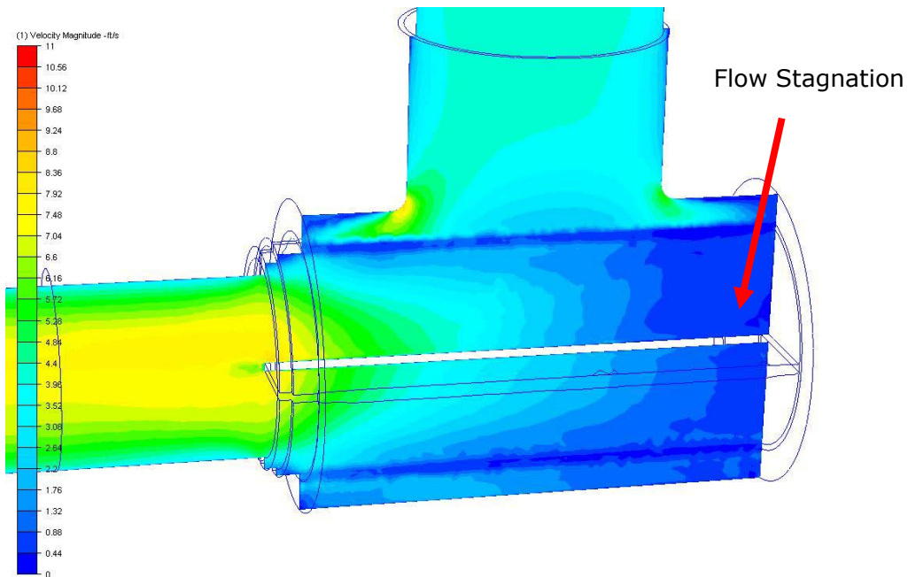
Figure 7. Cut-surface showing fluid velocity magnitude. (Cylindrical diffuser, 4 ft/s)
