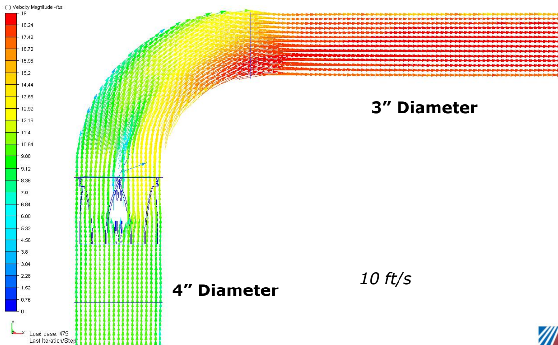
Figure 3. Cut-surface showing velocity vectors through the reducing elbow.
