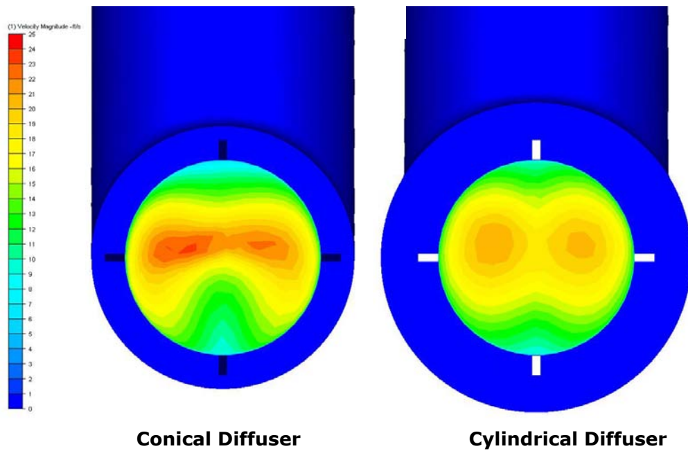
Figure 10. Fluid velocity profiles approximately 3 inches downstream of the diffuser screen.
