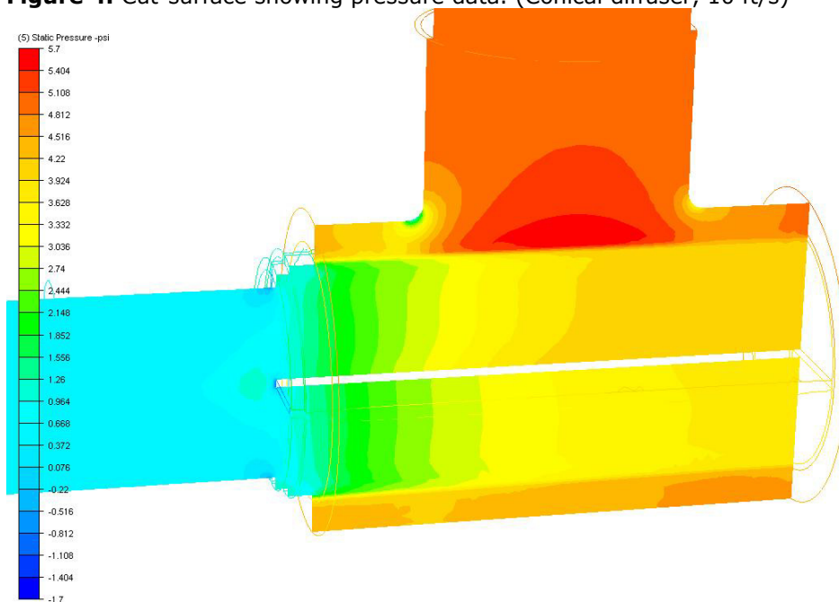
Figure 5. Cut-surface showing pressure data. (Cylindrical diffuser, 10 ft/s)
