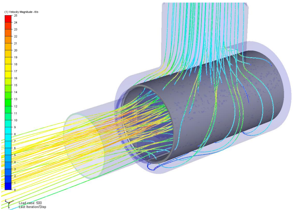
Figure 14. Fluid particle traces. (Cylindrical diffuser)
