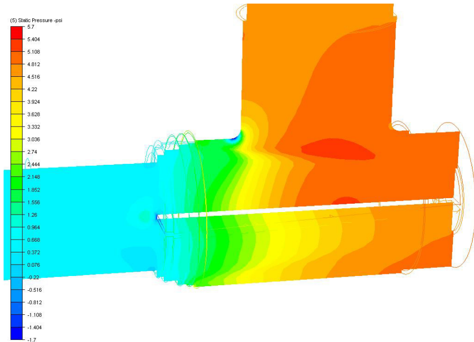
Figure 4. Cut-surface showing pressure data. (Conical diffuser, 10 ft/s)
