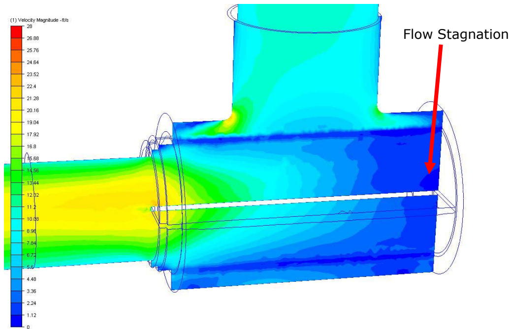
Figure 9. Cut-surface showing fluid velocity magnitude. (Cylindrical diffuser, 10 ft/s)
