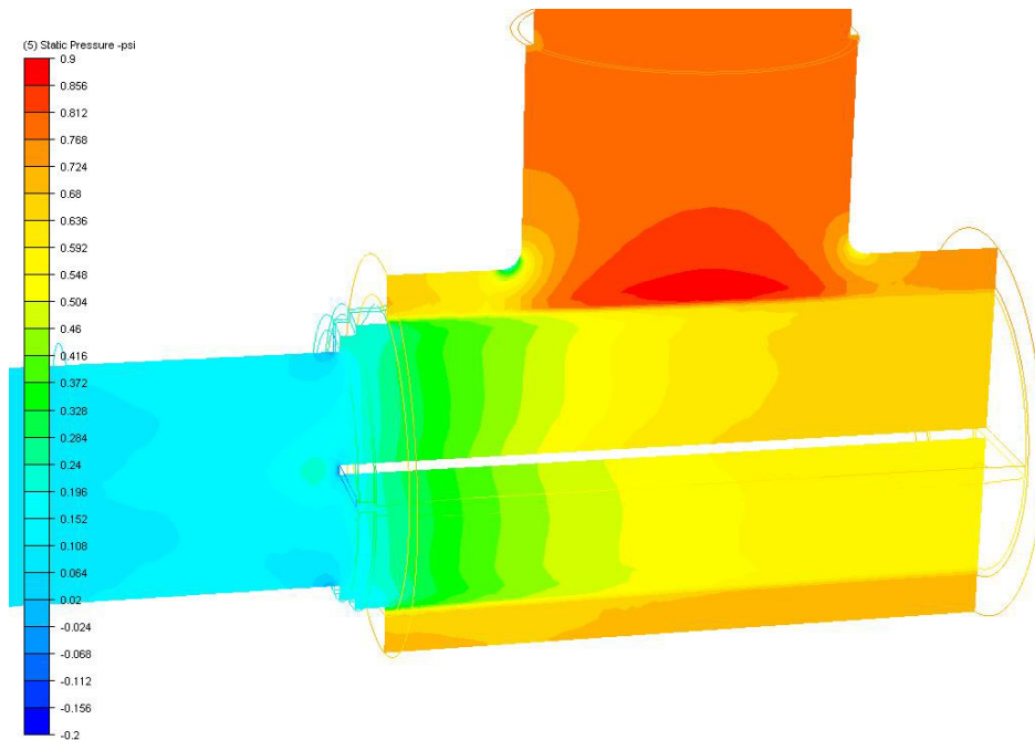
Figure 3. Cut-surface showing pressure data. (Cylindrical diffuser, 4 ft/s)
