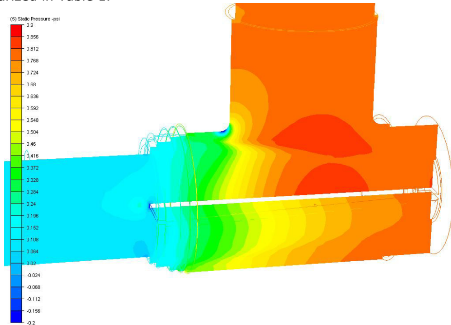
Figure 2. Cut-surface showing pressure data. (Conical diffuser, 4 ft/s)
