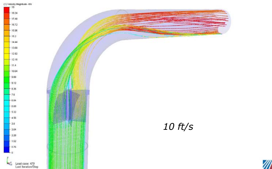
Figure 7. Fluid particle traces shown for the 10 ft/s flow rate.
