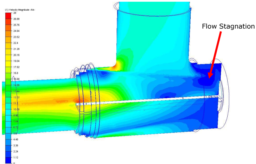
Figure 8. Cut-surface showing fluid velocity magnitude. (Conical diffuser, 10 ft/s)
