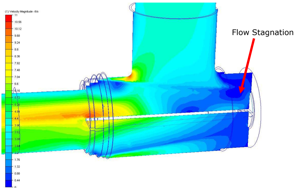
Figure 6. Cut-surface showing fluid velocity magnitude. (Conical diffuser, 4 ft/s)
