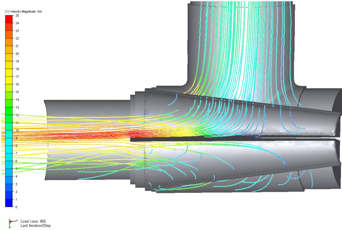
Figure 13. Fluid particle traces. (Conical diffuser)
