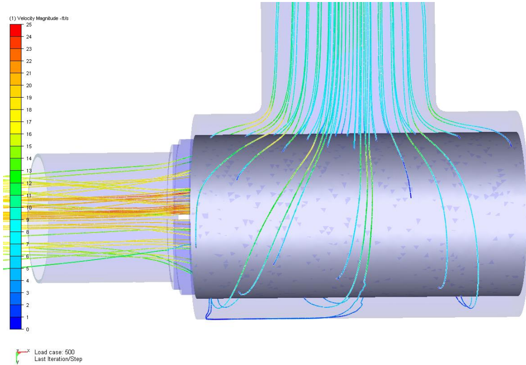
Figure 15. Fluid particle traces. (Cylindrical diffuser)
