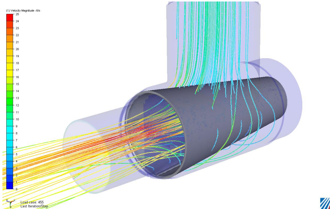
Figure 11. Fluid particle traces. (Conical diffuser)
