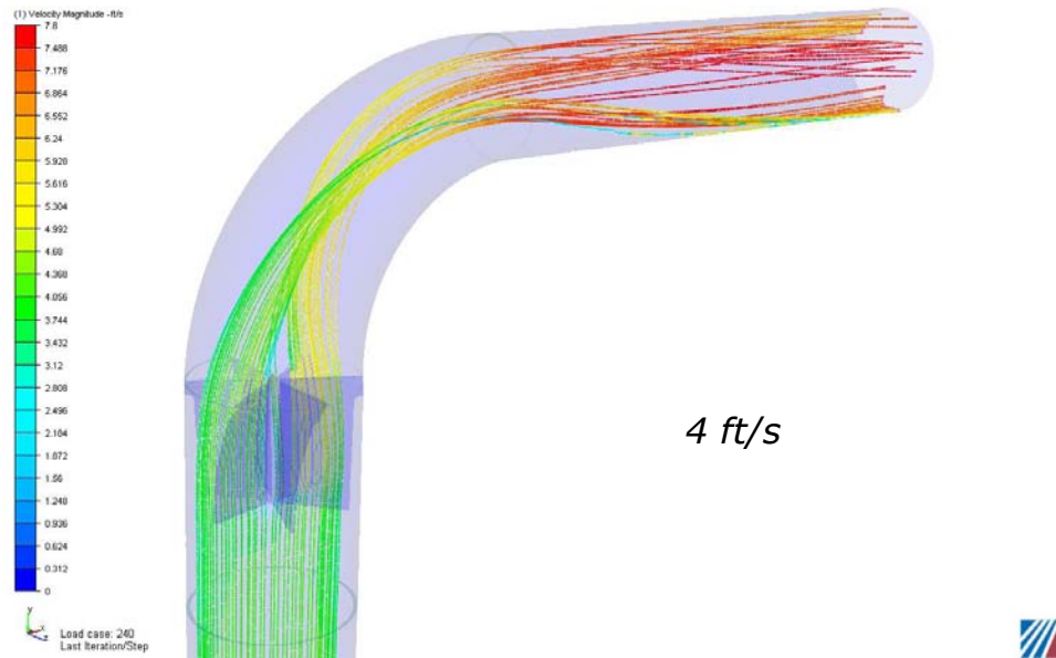
Figure 6. Fluid particle traces shown for the 4 ft/s flow rate.
