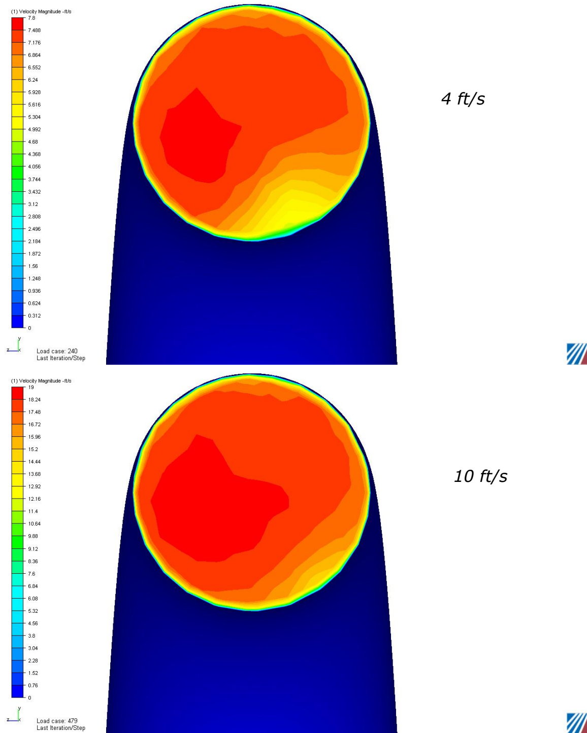
Figure 4. Velocity distribution normal to the flow 3" downstream of the elbow.
