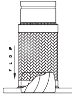
CRV Flex with 150# plate flange x groove end for connecting to a short radius elbow
