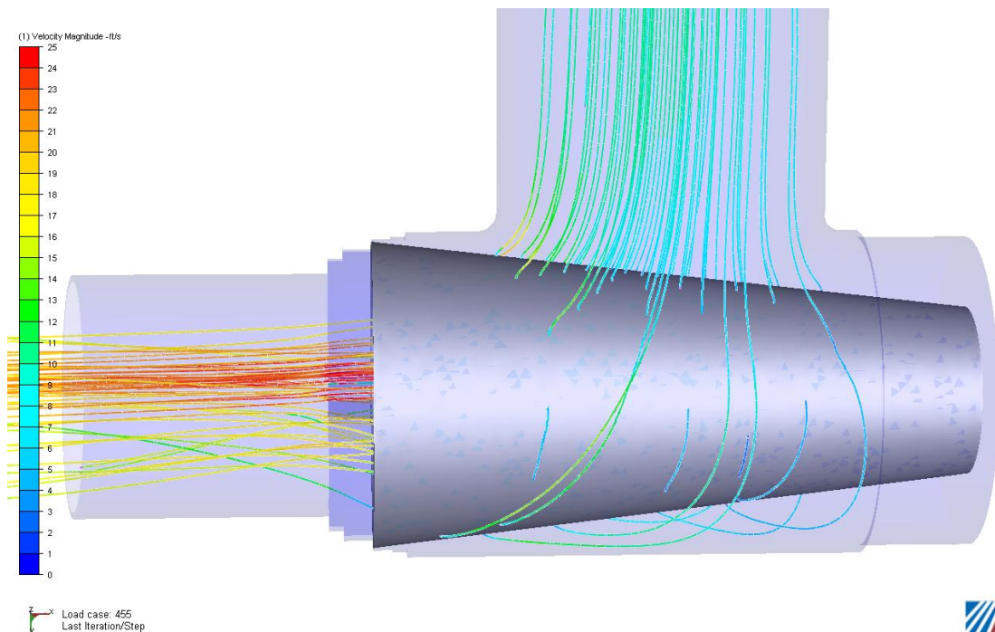
Figure 12. Fluid particle traces. (Conical diffuser)
