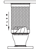
CRV Flex with 150# plate flanges with concentric reducer for connecting to a long radius elbow
