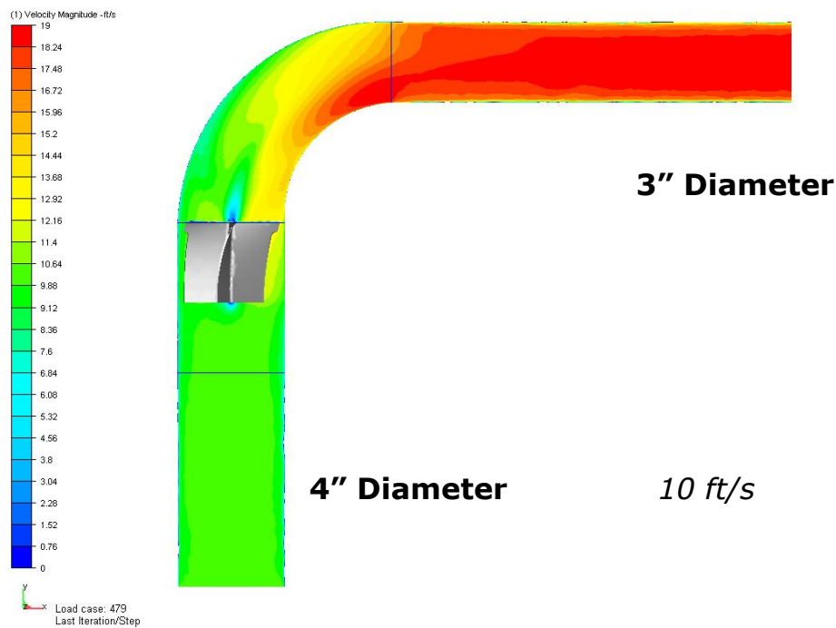
Figure 2. Cut-surface showing velocity contours through the reducing elbow.
