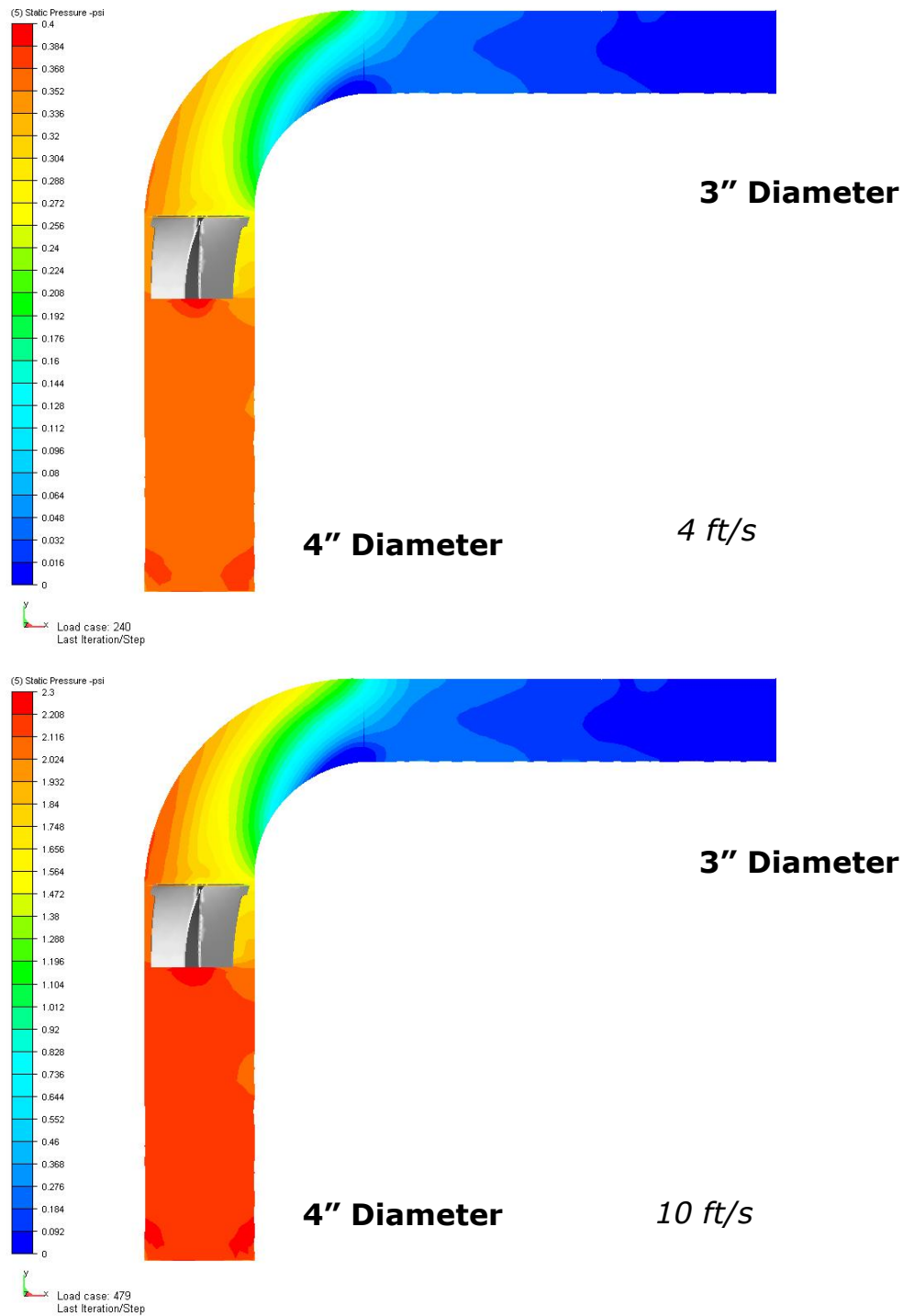
Figure 5. Cut-surface showing pressure gradients through the elbow.
